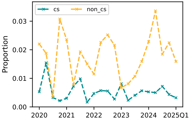
Function Names - single_letter
